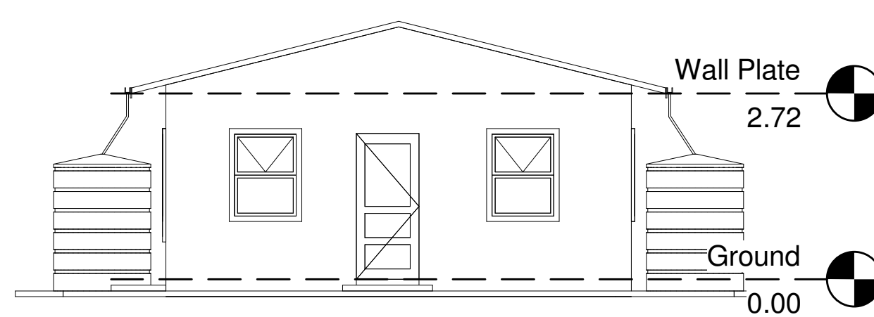
4 EAST ELEVATION 1 : 100
