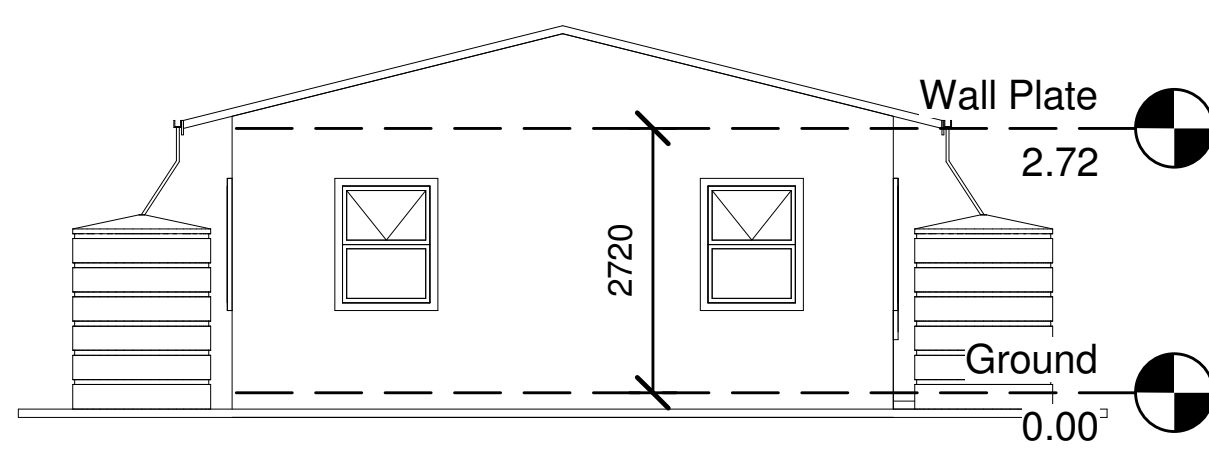
5 WEST ELEVATION 1 : 100
