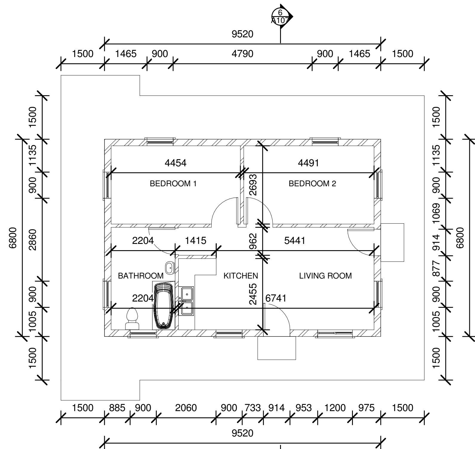
1 GROUND FLOOR 1 : 100
