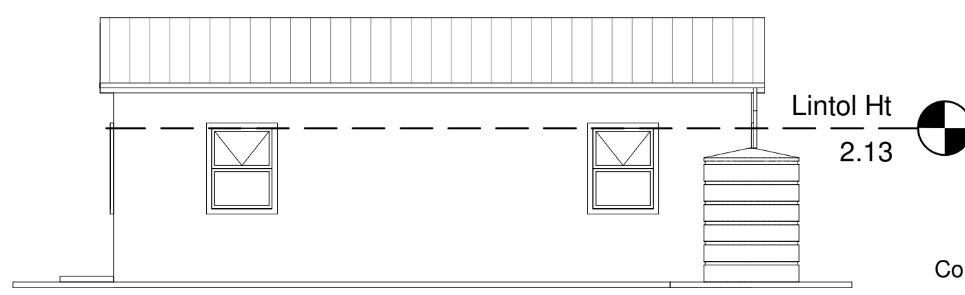
2 NORTH ELEVATION 1 : 100
