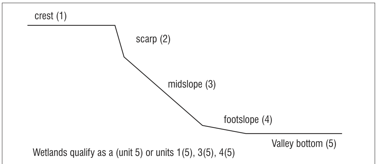
Figure 2: Terrain Units
