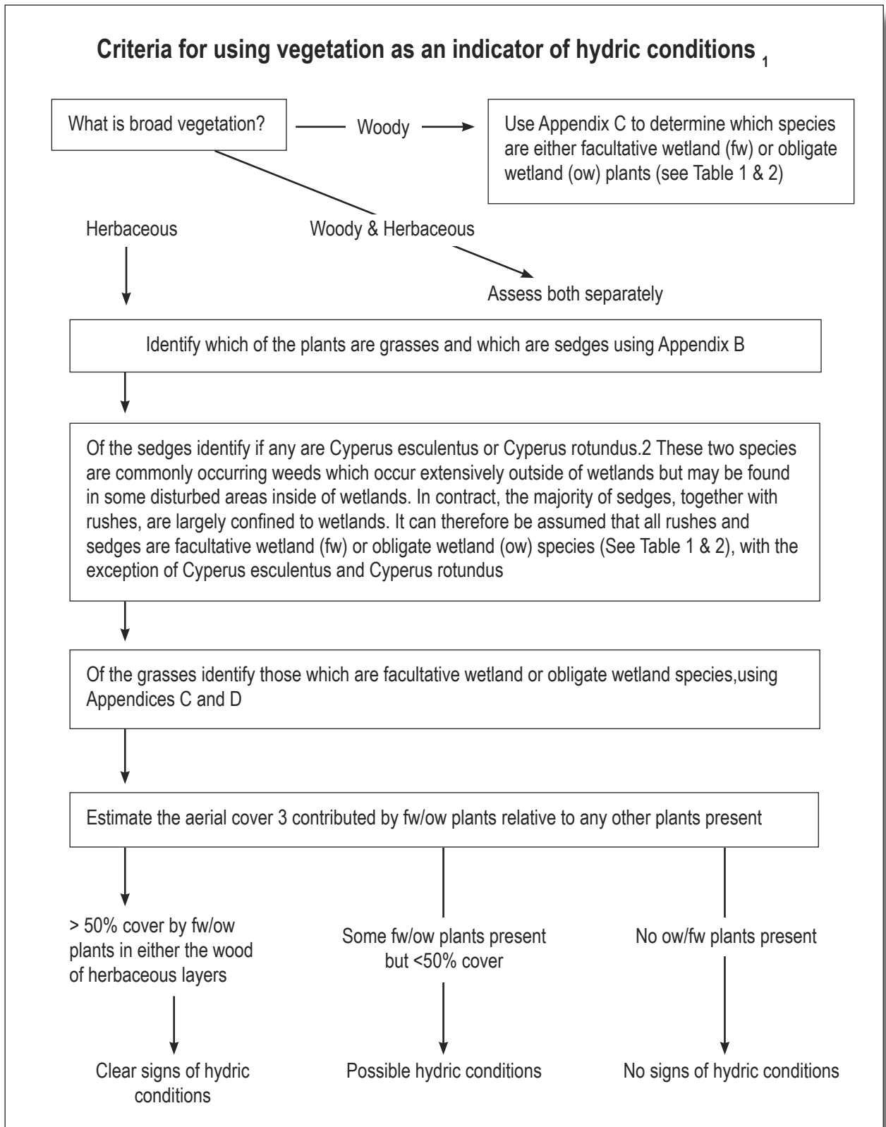
Figure 3: Method for utilising vegetation as an indicator of wetland conditions (Kotze and Marnebeck, 1999)
