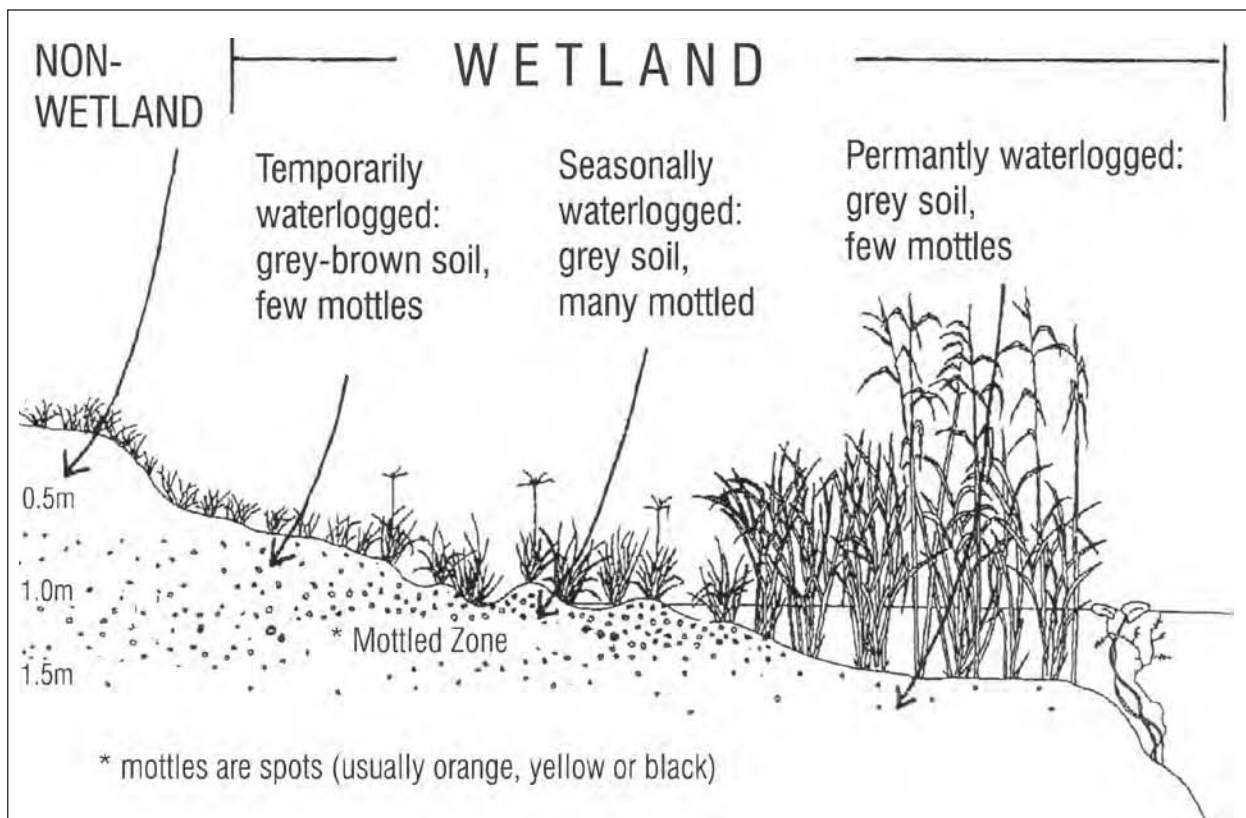
Figure 1: Cross section through a wetland, indicating how the soil wetness and vegetation indicators change as one moves along a gradient of decreasing wetness, from the middle to the edge of the wetland.
