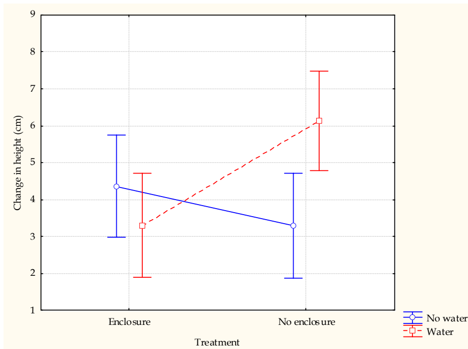
Figure 1 Least Square Means plot showing interaction between water and enclosure effects. Vertical bars denote 0.95 confidence intervals; F(1.006) = 7.7356 ; p < 0.01 .
